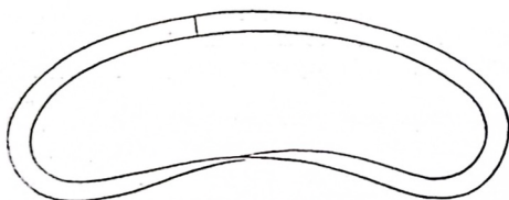
Möbius' Ring.
